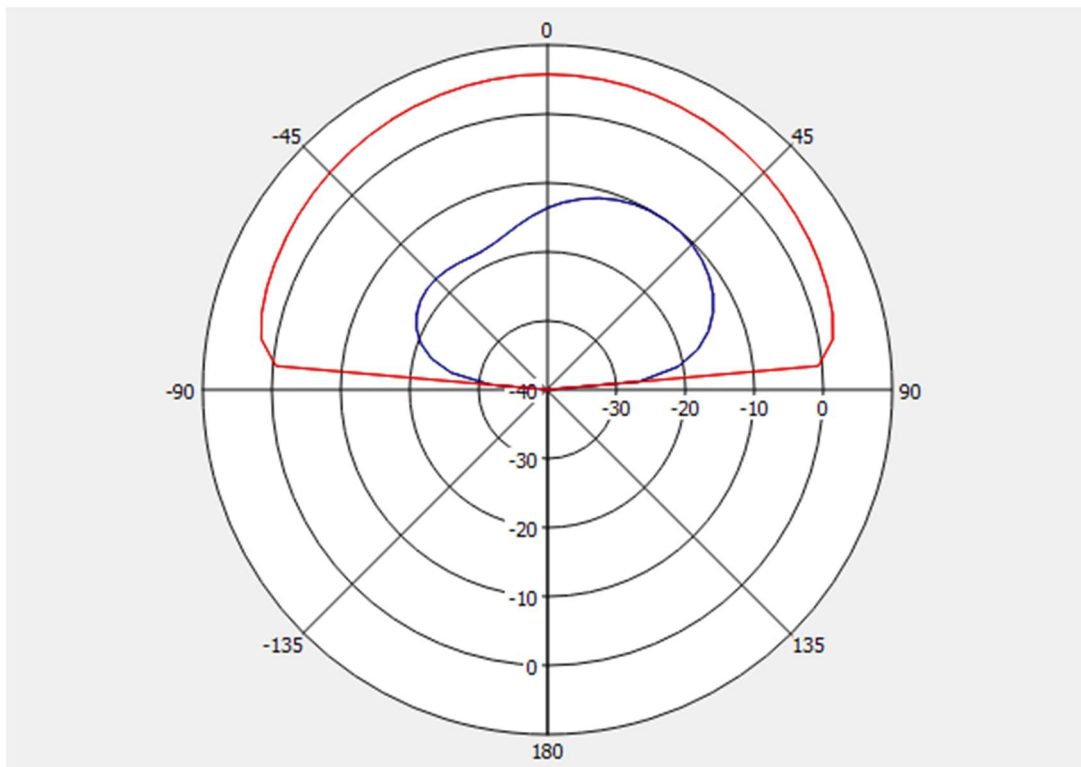
Figure 5. Polar plot for antenna
