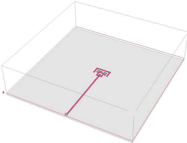
Figure 2. 3D antenna topology
