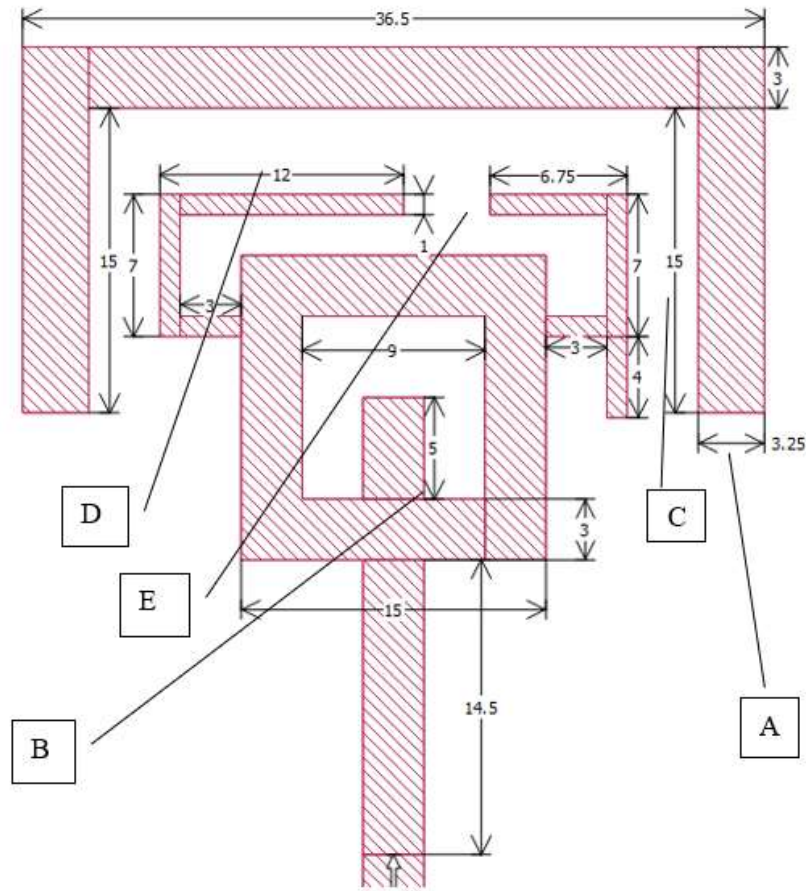
Figure 1. Antenna topology
