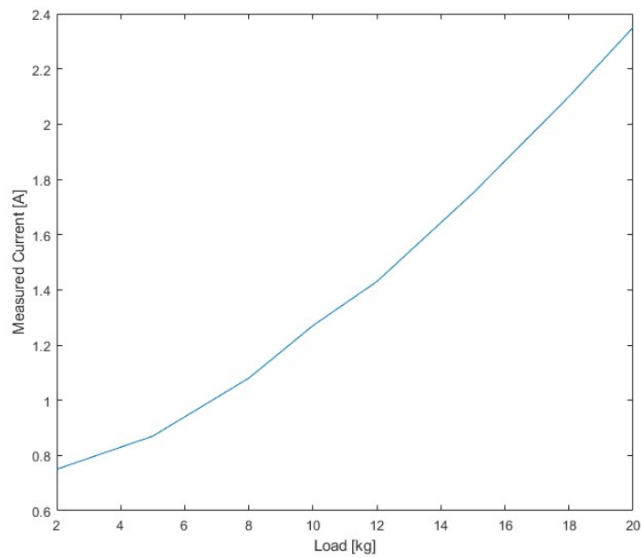
Figure 4. Current consumption vs. load values
