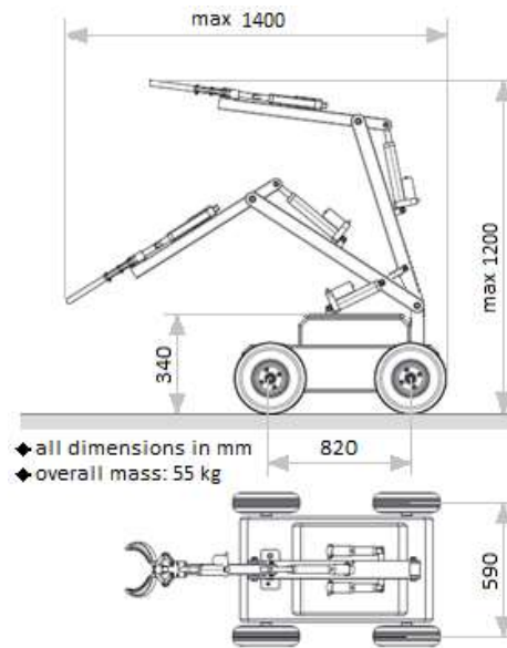
Figure 2. Dimensional sketch of the robot
