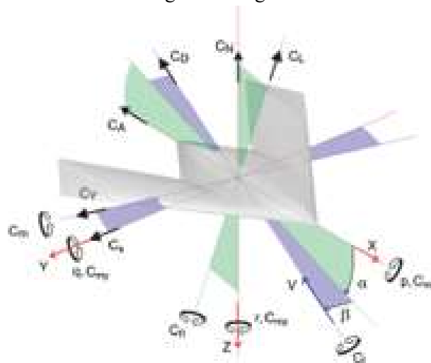
Figure 9. Coordinate System of SACCON UCAV
