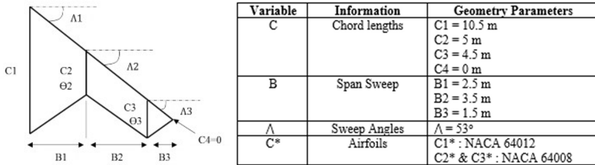
Figure 7. SACCON UCAV Geometry Parameterization
