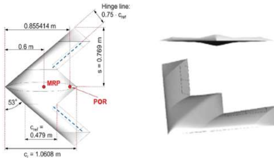
Figure 8. Design of SACCON UCAV
