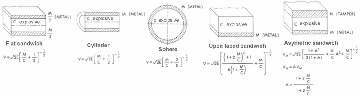
Fig. 2 Expressions for initial velocities of fragments in different geometric configurations [2]
