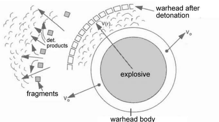
Figure 1. Schematic representation of the HE warhead detonation process [12]
