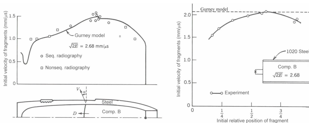
Figure 3. Comparison of the Gurney method with experimental data [2]
